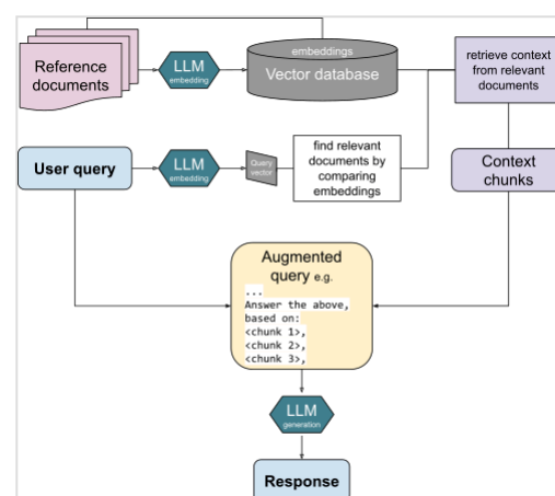
Overview of RAG process, combining external documents and user input into an LLM prompt to get tailored output
